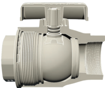
Double seal on spindle to prevent leakage
